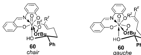
Figure 6. Proposed binding modes of the tert -butylperoxy ligand and 5-methyl-1-phenylhex-4-en-1-ol ( 5 ) in vanadium(v) complex 60 ; R^E = R^Z = \text{methyl}
