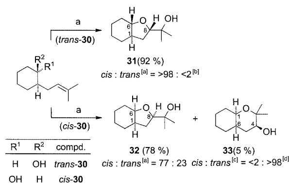
Scheme 3. Formation of bicyclic compounds from both diastereomers of 2-allyl-substituted bicyclic cyclohexanol 30 ; reagents and conditions: (a) 1.5 equiv. TBHP, 10 mol % VOL 7 (OEt) ( 4g ), CHCl 3 , 20 °C, 48 h; [a] stereodescriptors cis and trans refer to relative configurations at C6 and C8; [b] corresponding trans isomer was not detected ( 1 H NMR spectroscopy); [c] stereodescriptors cis and trans refer to relative configurations at C1 and C4; [d] corresponding cis isomer was not detected ( 1 H NMR spectroscopy)
