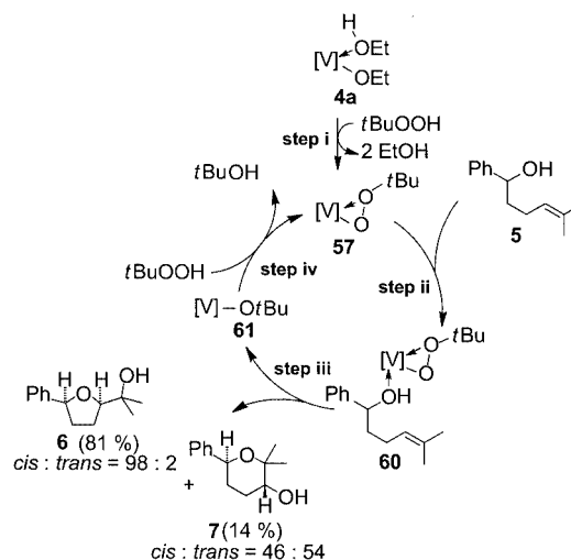
Scheme 8. Proposed catalytic cycle for the synthesis of cyclic ethers 6 and 7 in a (Schiff-base)vanadium(v) complex catalyzed oxidation of methyl-phenylhexenol 5
