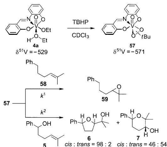
Scheme 6. Formation of peroxy complex 57 (top) and its use in competition kinetic investigations (bottom)
