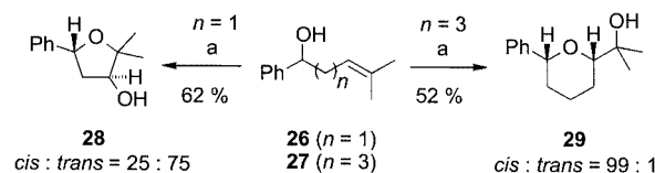
Scheme 2. Stereoselective synthesis of functionalized cyclic ethers 28 and 29 ; reagents and conditions: (a) 1.5 equiv. TBHP, 10 mol % VOL 7 (OEt) ( 4g ), CHCl 3 , 20 °C, 48 h
