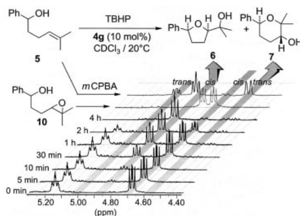
Figure 4. Stacking plot from a time-dependent 1 H NMR investigation of the oxidation of methyl-phenylhexenol 5 with TBHP in the presence of (Schiff-base)vanadium(v) complex 4g ; the selected spectral region depicts resonances of the olefinic and the benzylic proton in substrate 5 ( t = 0 min) and benzylic protons of cyclic ethers 6 and 7 (see t = 4 h); for illustration purposes, 1 H NMR spectra of a 1:1 mixture of like - and unlike -configured diastereomers of epoxy alcohol 10 and a crude reaction mixture, which had been obtained from an m CPBA-mediated oxidation of bis-(homoallylic) alcohol 5 , have been added to this plot
