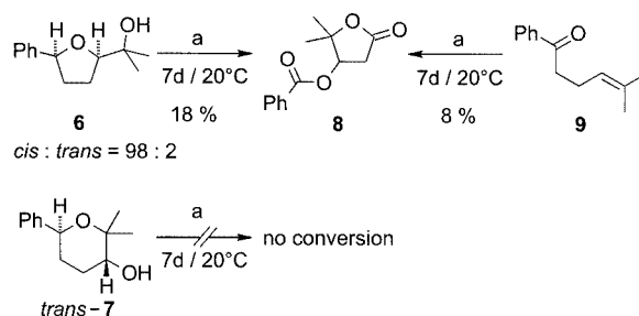
Scheme 1. Control experiments for investigating the stability of oxidation products; reagents and conditions: (a) 1.5 equiv. TBHP, 10 mol % VOL 1 (OEt)(EtOH) ( 4a )
