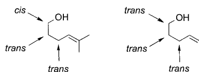
Figure 8. Guidelines for the stereoselective synthesis of functionalized tetrahydrofurans from substituted bis(homoallylic) alcohols
