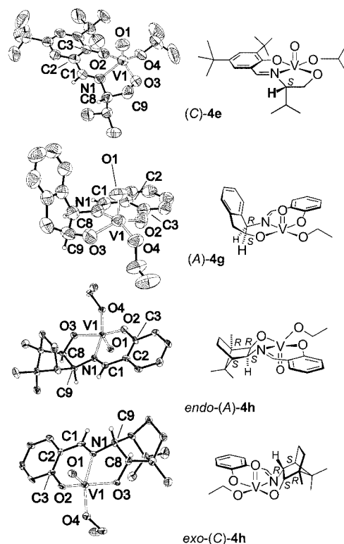
Figure 3. Solid-state structures of (Schiff-base)vanadium(v) complexes 4e , 4g , and 4h (anisotropic displacement parameters drawn at the 50% probability level) showing labeling of selected non-H atoms; selected hydrogen atoms are depicted as circles of an arbitrary radius
