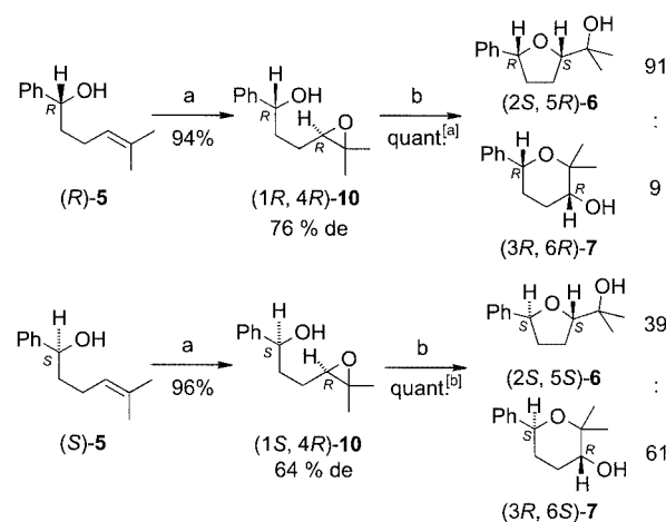
Scheme 7. Diastereoselective conversion of alkenols ( R )- 5 and ( S )- 5 into corresponding cyclic ethers 6 and 7 ; reagents and conditions: (a) Shi epoxidation; [49] (b) TsOH (1 equiv. or 4g (0.1 equiv.)); [a] yields: 80% of (2 S ,5 R )- 6 , 8% of (3 R ,6 R )- 7 , and 12% of a 39:61 mixture of trans - 6 and trans - 7 ; [b] yields: 32% of (2 S ,5 S )- 6 , 50% of (3 R ,6 S )- 7 , and 18% of a 91:9 mixture of cis - 6 and cis - 7
