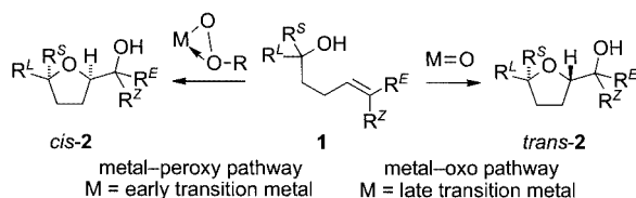
Figure 1. Mechanisms for diastereoselective syntheses of functionalized tetrahydrofurans 2 from bis(homoallylic) alcohols 1 ; R^S = small substituent, R^L = large substituent, R^Z = alkyl substituent in ( Z ) arrangement, R^E = alkyl substituent in ( E ) arrangement, R = C(CH_3)_3 , C(CH_3)_2C_6H_5
