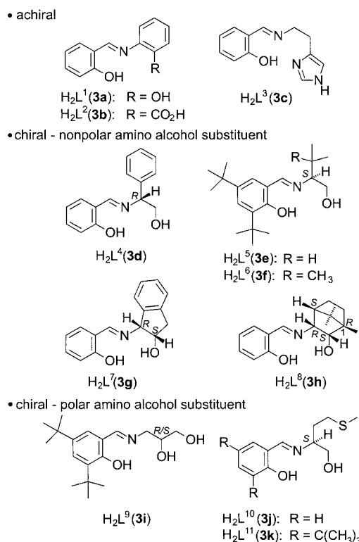
Figure 2. Structural formulae of Schiff-base auxiliaries 3a–k for the synthesis of derived vanadium(v) complexes 4a–k (see Table 1)
