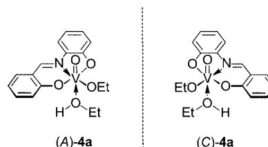
Figure 5. Geometry of (Schiff-base)vanadium(v) complex ( A )- 4a (left) and its enantiomer ( C )- 4a (right) [31]
