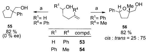
Scheme 5. Conversion of 4-substituted bis(homoallylic) alcohols 53 and 54 into cyclic ethers 55 and 56 ; reagents and conditions: (a) 1.5 equiv. TBHP, 10 mol % VOL 7 (OEt) ( 4g ), CHCl 3 , 20 °C, 48 h
