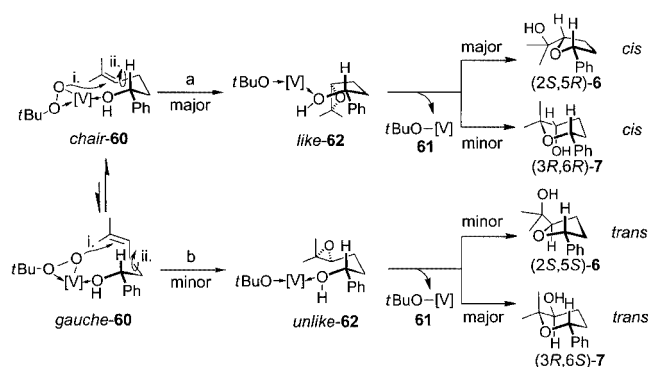
Figure 7. Stereochemical model for correlating the facial selectivity of \pi -bond oxygenation from “loaded” peroxy complex 60 with the geometry of similarly prepared cyclic ethers 6 and 7
