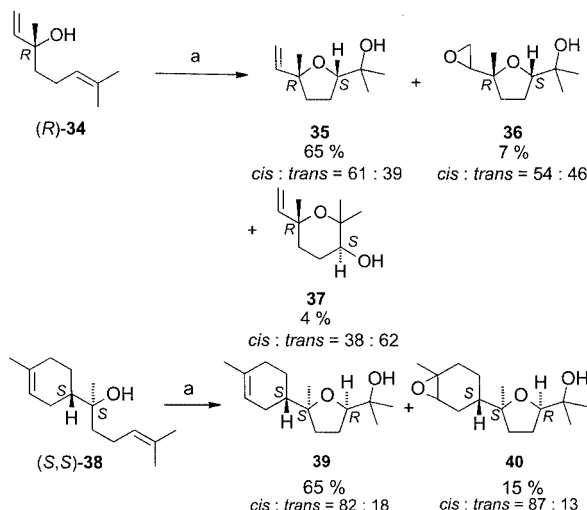
Scheme 4. Vanadium(v)-catalyzed oxidation ( R )-linalool [( R )- 34 ] and ( S,S )-bisabolol [( S,S )- 38 ]; reagents and conditions: (a) 1.5 equiv. TBHP, 10 mol % VOL † (OEt) ( 4g ), CHCl 3 , 20 °C, 48 h
